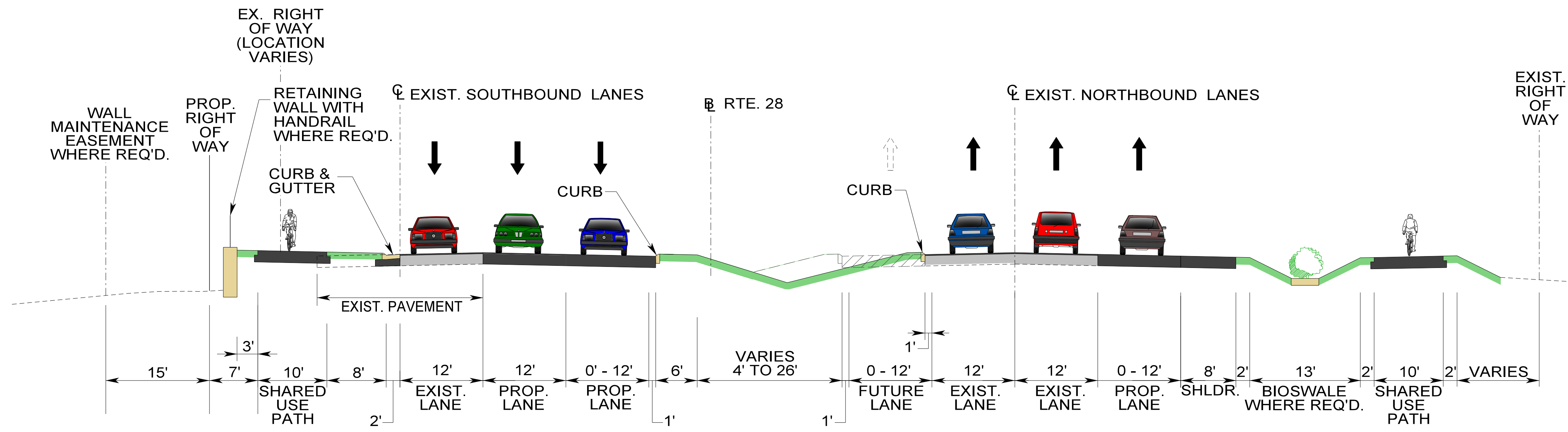
TYPICAL TRANSITION SECTION (BRIDGE OVER BULL RUN TO COMPTON ROAD)
