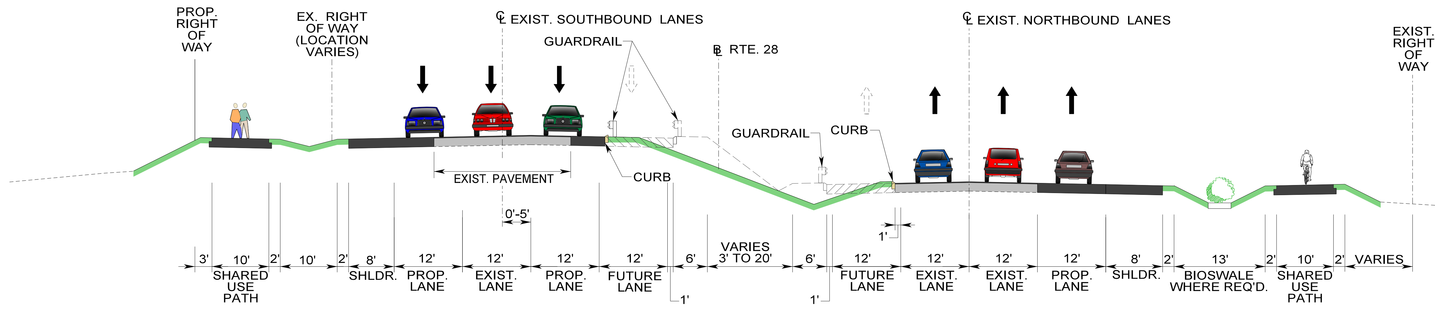
TYPICAL SECTION (WITH OUTSIDE SHOULDERS) (COMPTON ROAD TO 100' SOUTH OF DARKWOOD DRIVE)
