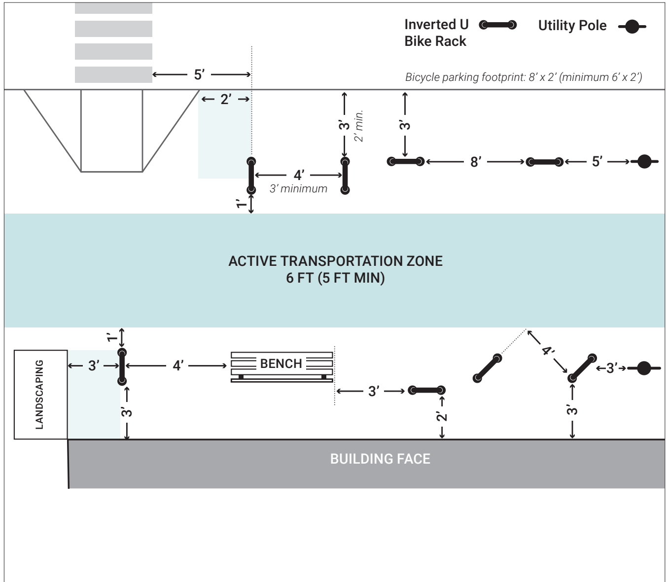
Figure 3. Bike Parking Site Planning for Inverted U Bicycle Racks
