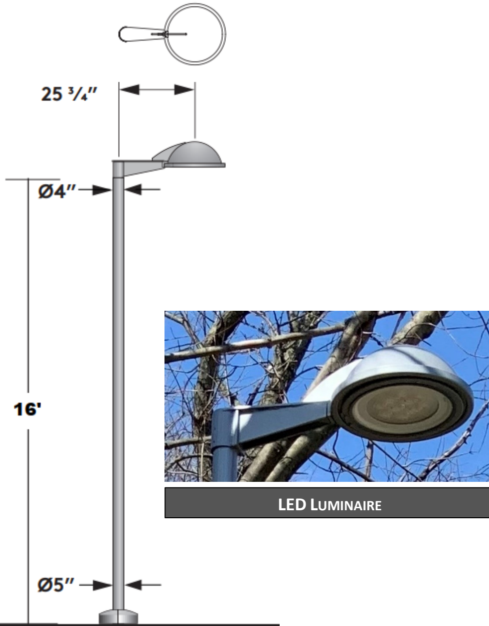
TAPERED POLE AND LIGHTING FIXTURES DIMENSIONS
