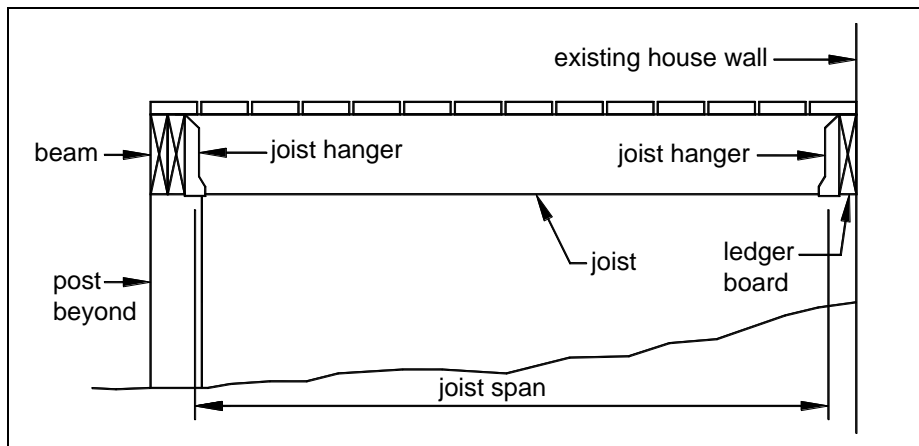
FIGURE 3: JOIST SPAN - JOISTS ATTACHED TO SIDE OF BEAM
