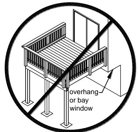
FIGURE 19: HOUSE OVERHANG
