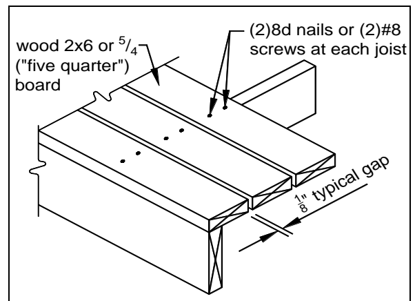
FIGURE 1: TYPICAL DECKING
