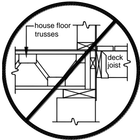
FIGURE 17: FLOOR TRUSSES
