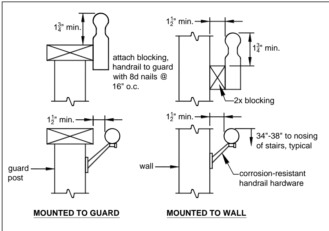
FIGURE 39: HANDRAIL REQUIREMENTS
