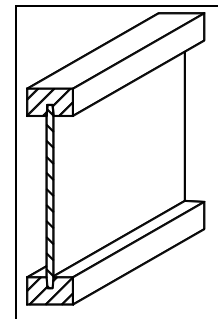
FIGURE 13: WOOD I-JOIST PROFILE
