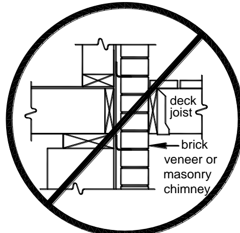
FIGURE 18: BRICK VENEER
