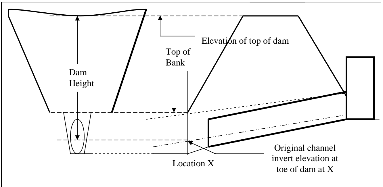
Figure 2: Front elevation and Profile of Dam Superimposed on Original Channel
