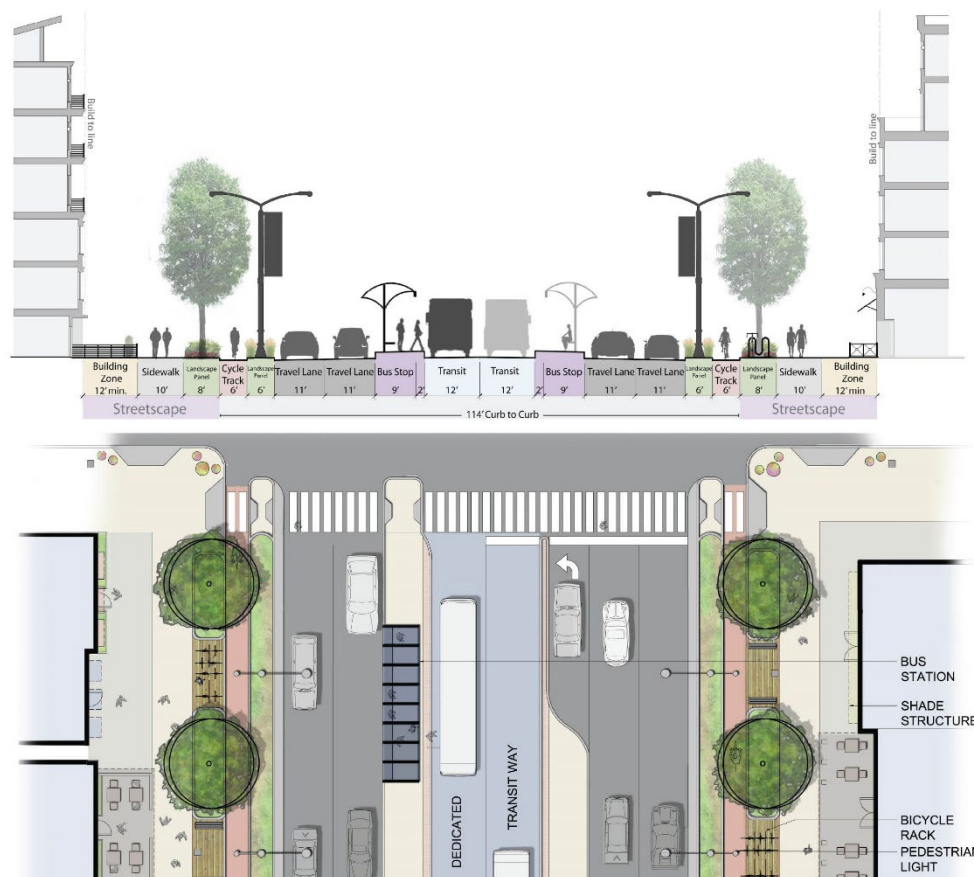
Figure 34 – Transit Boulevard Median Running Cross-section
