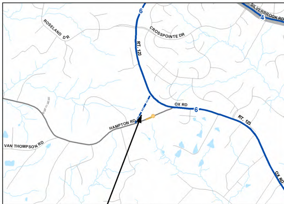
REALIGN HAMPTON ROAD AT ROUTE 123
