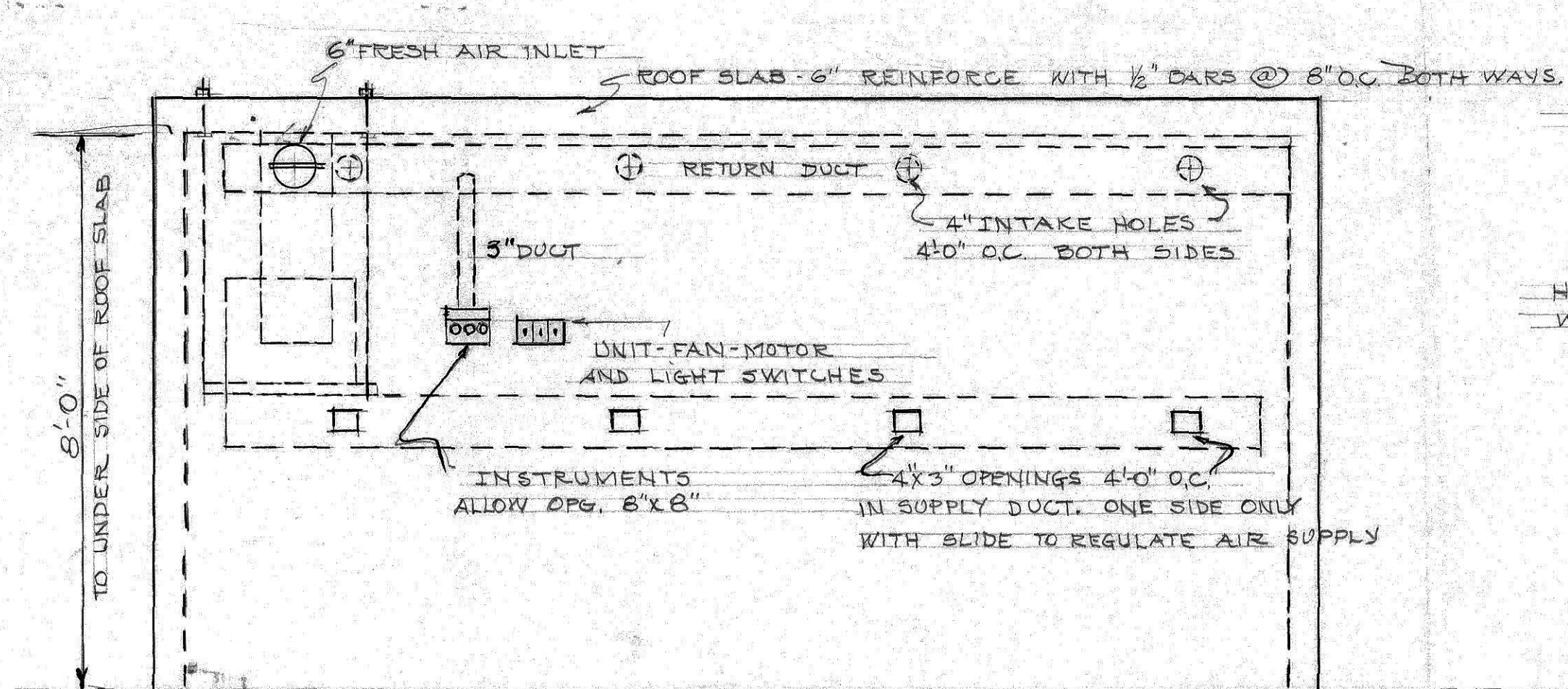
SIDE ELEVATION
