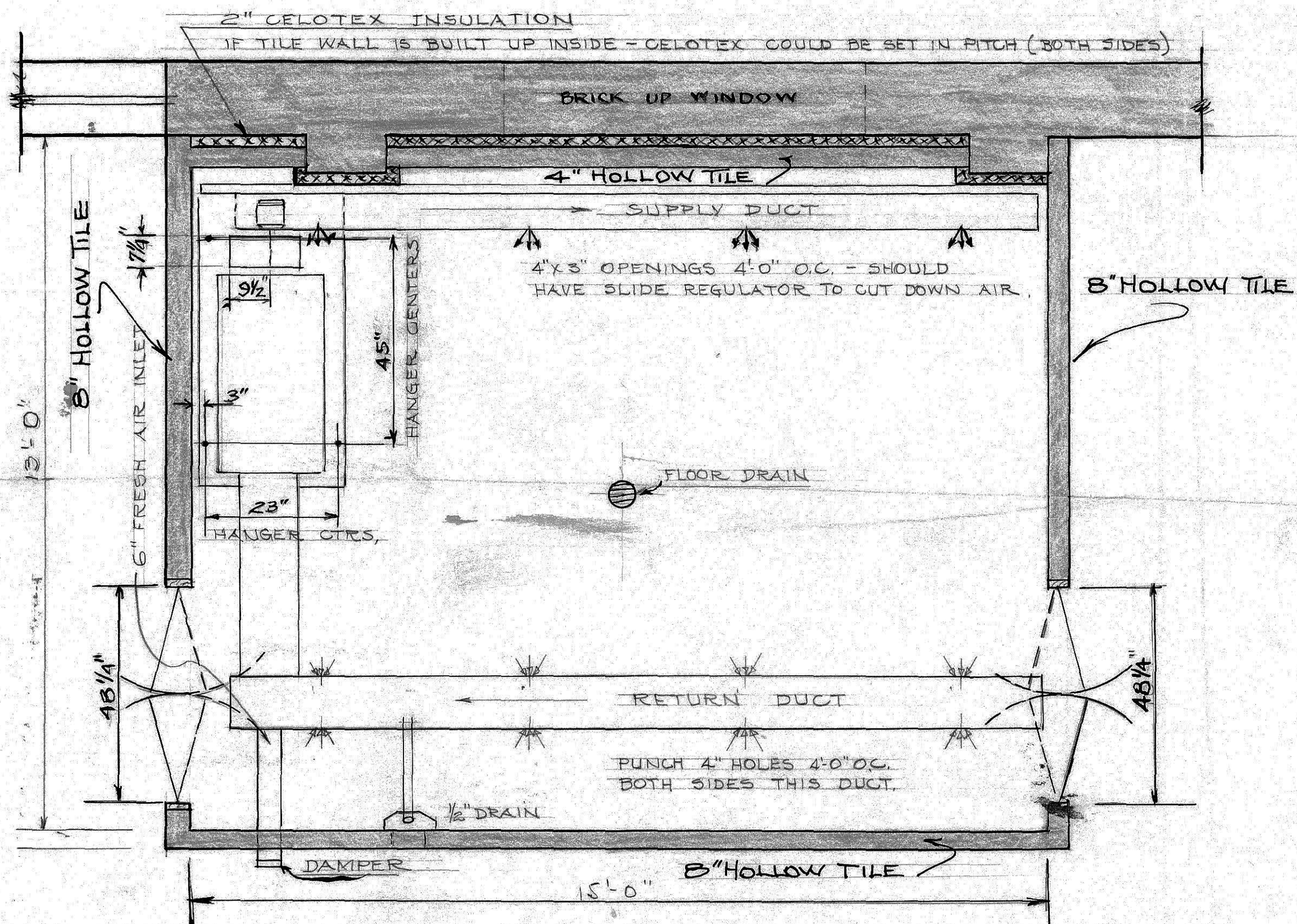
PLAN
