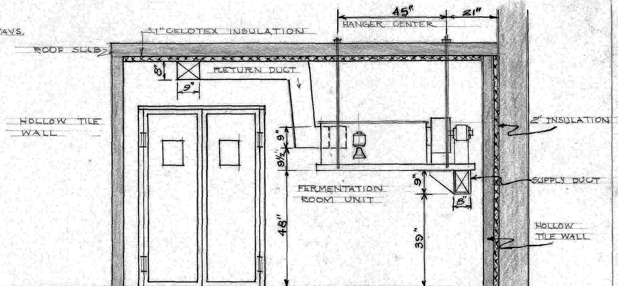
SECTION
