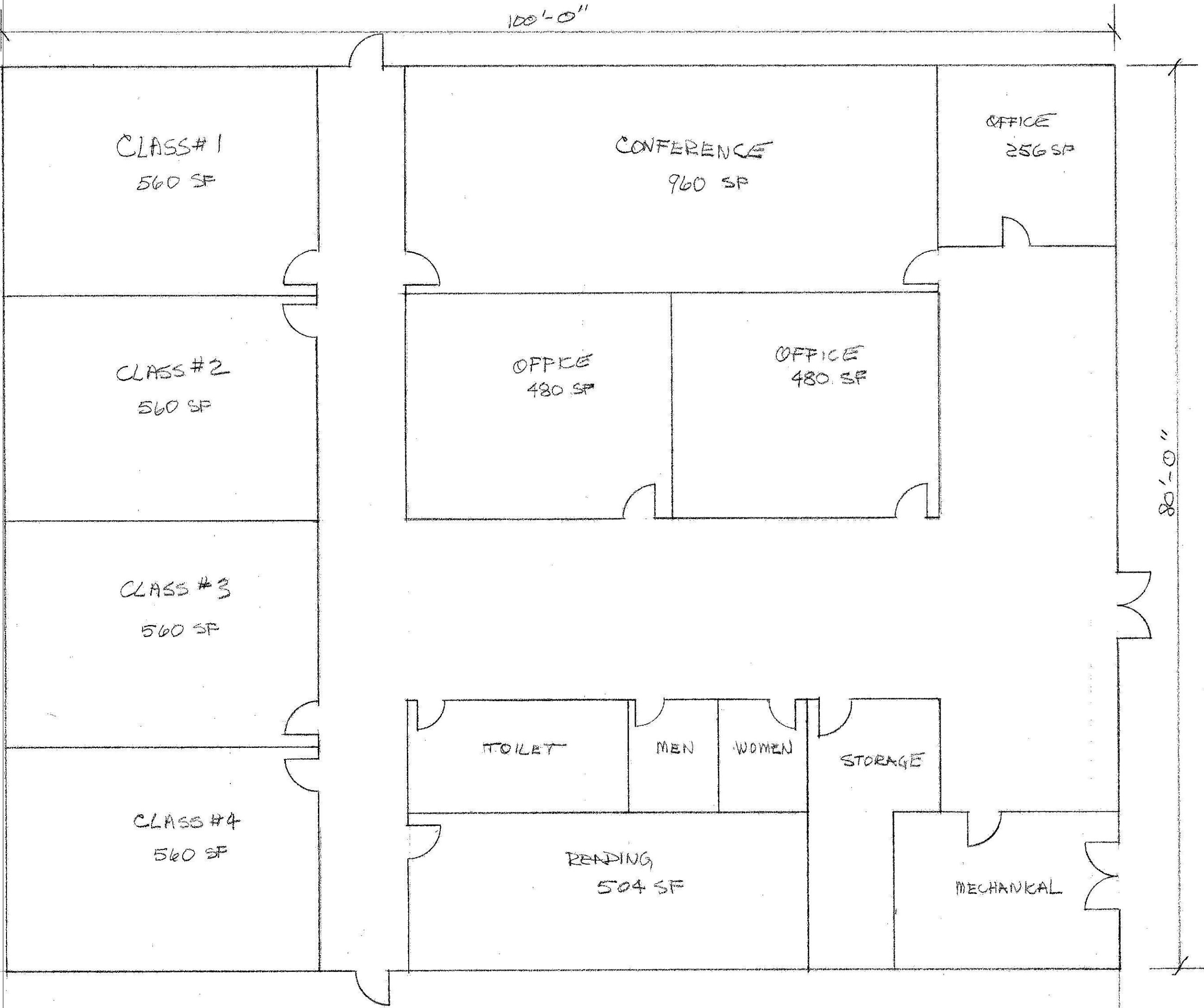
CENTRAL FACILITY SCALE \frac{1}{8}" = 1'-0"
