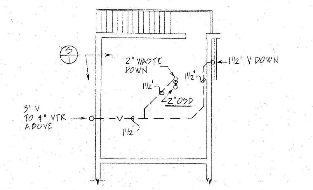
MECHANICAL RM.-PLUMBING SCALE 1/8"=1'-0"
