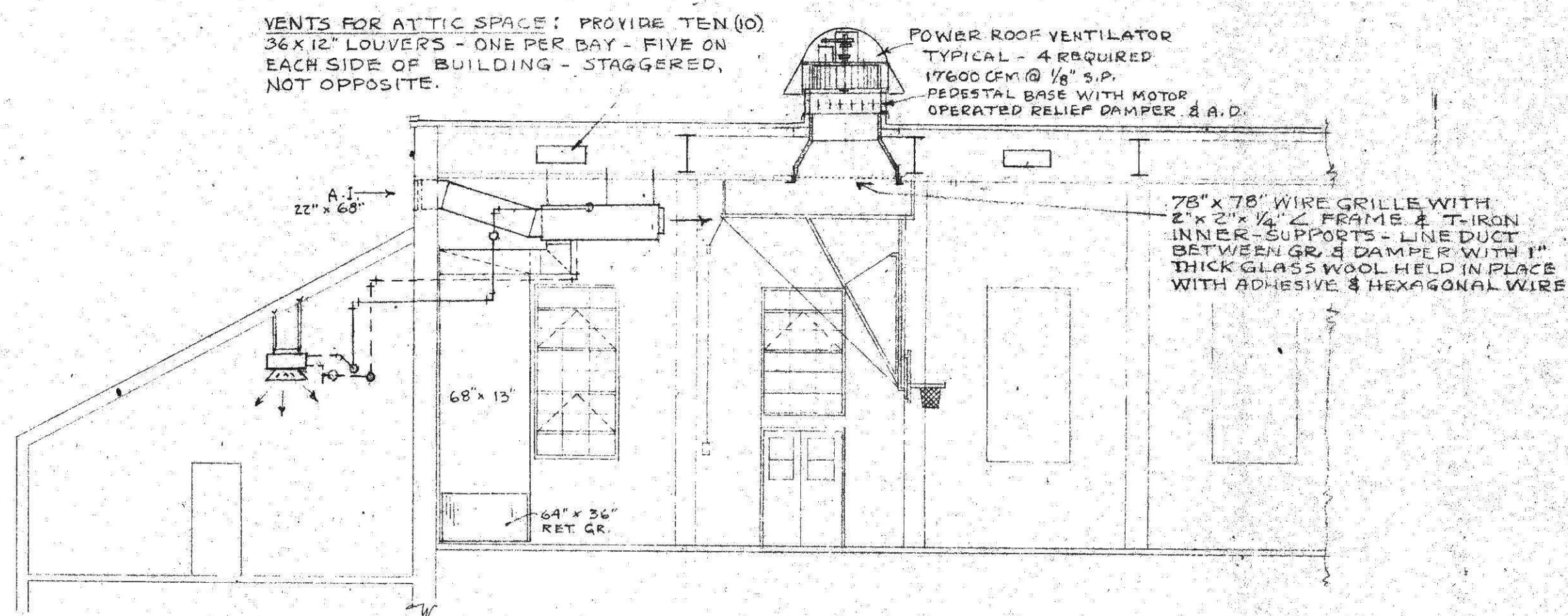
SECTION A-A NORTH END SCALE 1/8" = 1'-0"
