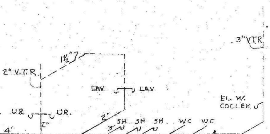
PLUMBING RISER DIAGRAM NO SCALE
