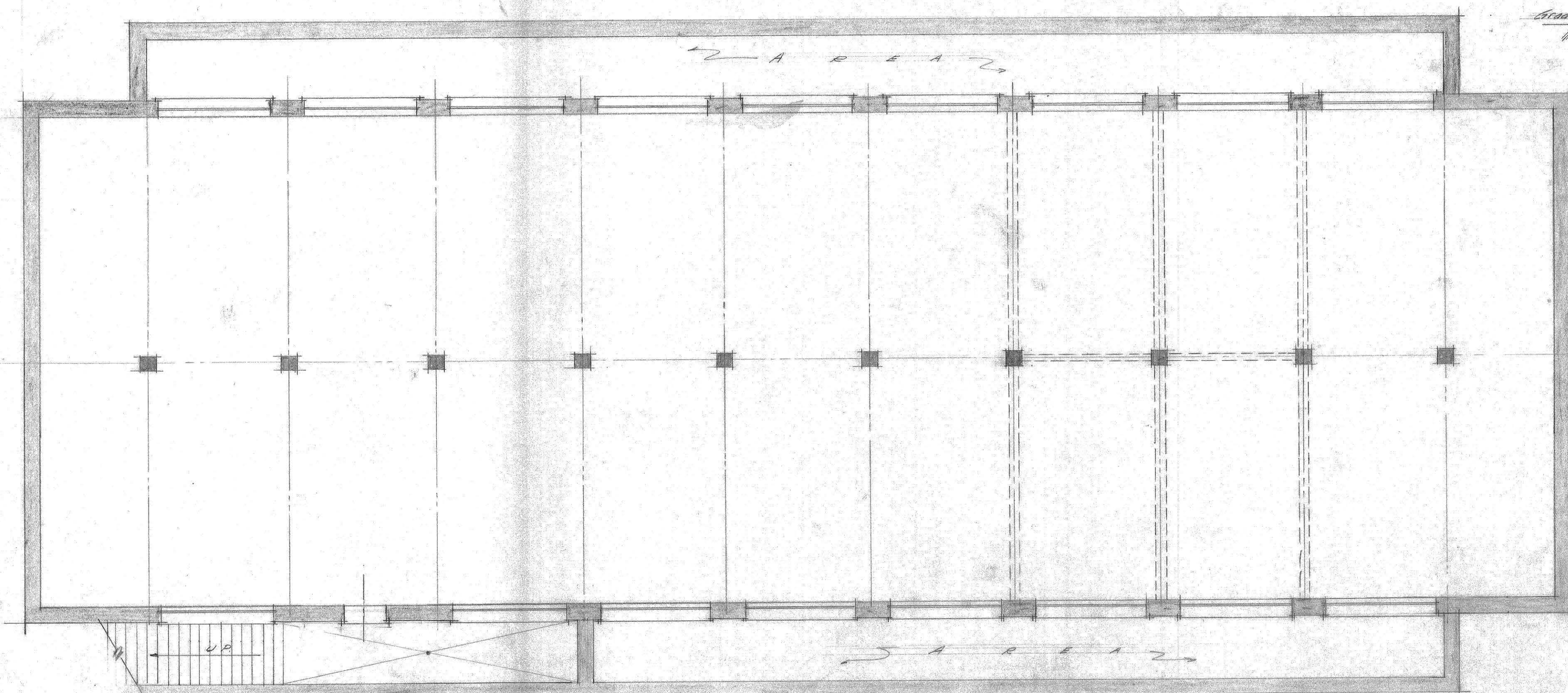
BASEMENT PLAN
