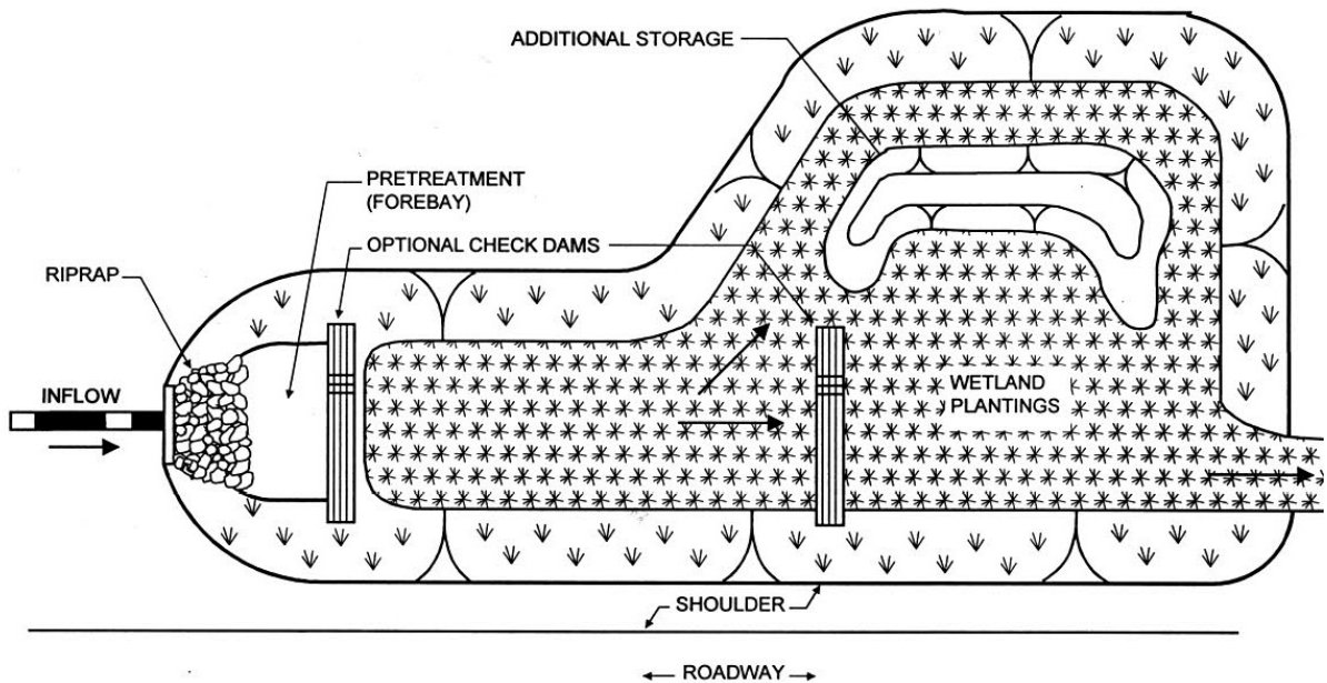
Figure 3.11: Wet Swale
