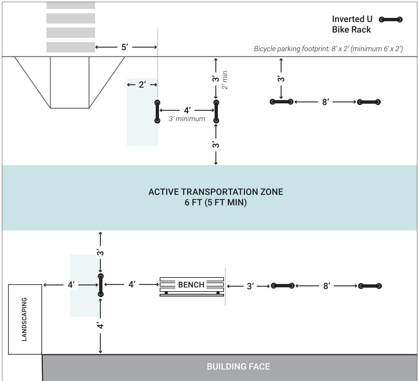
Figure 3. Bike Parking Site Planning for Inverted U Bicycle Racks
