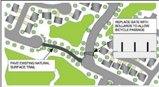
Figure 12: Bicycle link concept Source: Toole Design Group.
