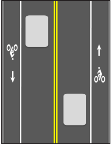
Figure 1: Bicycle lane concept Source: Toole Design Group.
