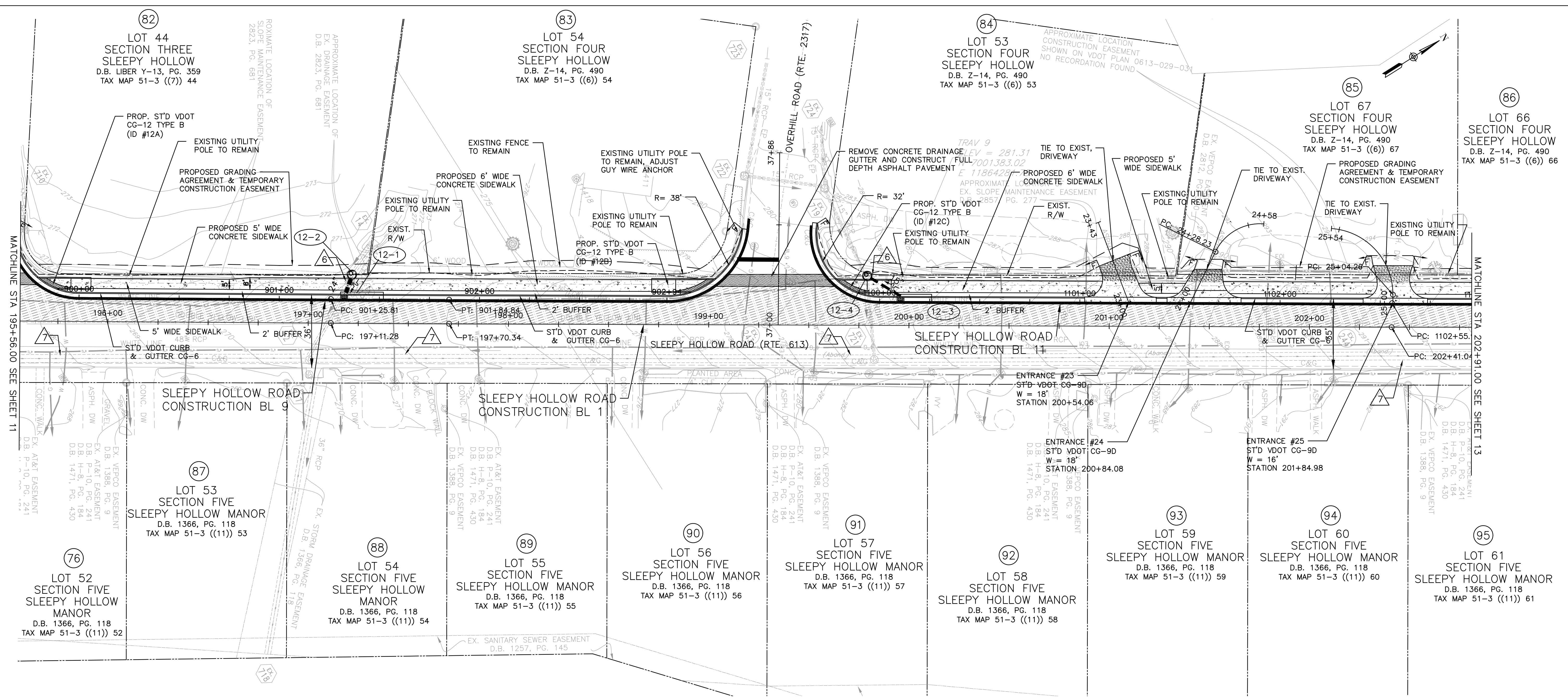
PLAN VIEW SCALE: 1"=25'
