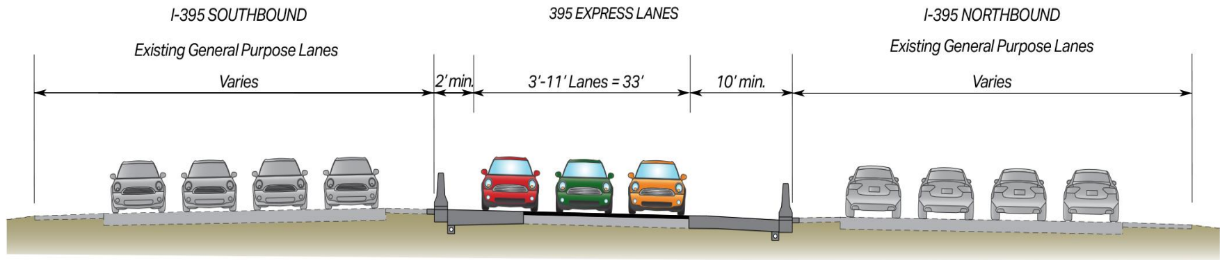
Typical Project Cross Section
