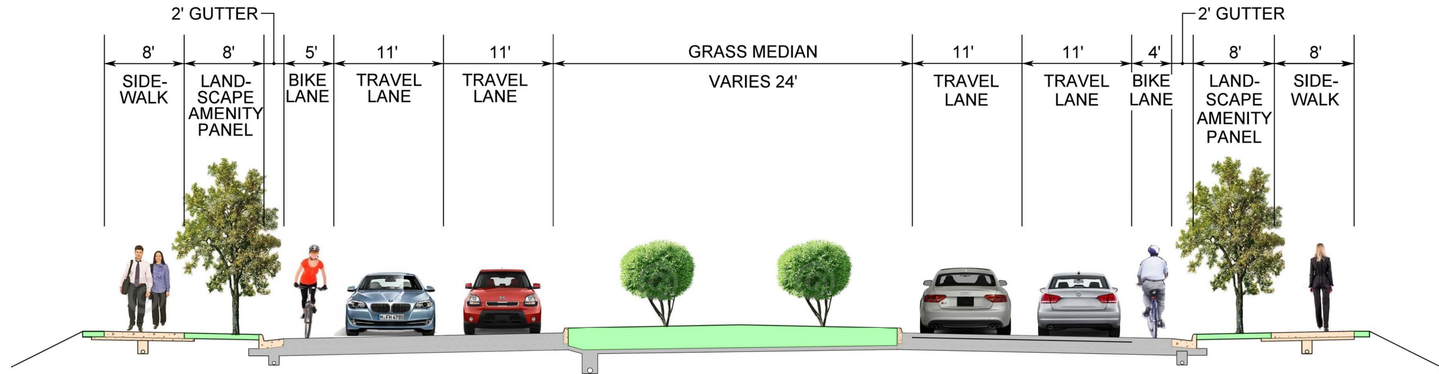
JONES BRANCH CONNECTOR - ROADWAY
