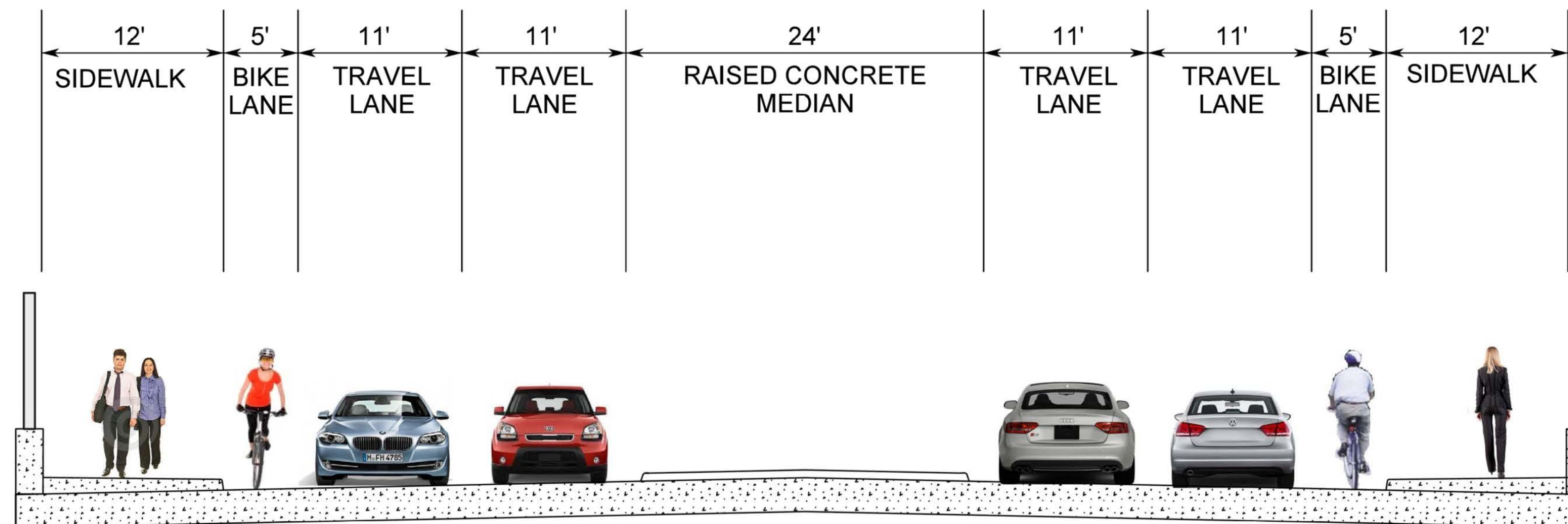
JONES BRANCH CONNECTOR - BRIDGE OVER I-495 NB
