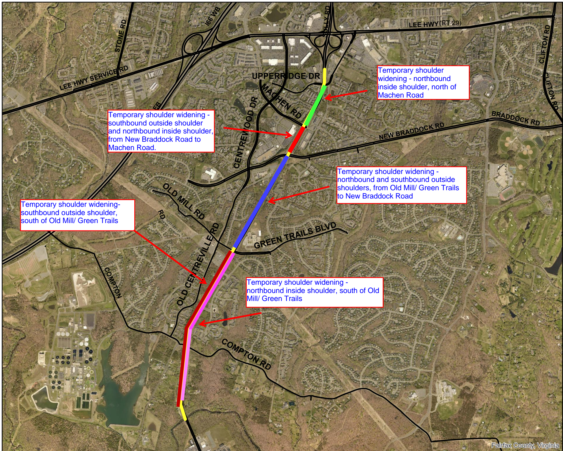
ROUTE 28 TEMPORARY SHOULDER WIDENING- SOUTH OF COMPTON ROAD TO SOUTH OF ROUTE 29 ---VDOT PROJECT 0028-029-269, UPC 108720
